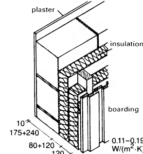
⑧ Walling with applied sheathing 0.11-0.19 W/(m 2 ·K)
